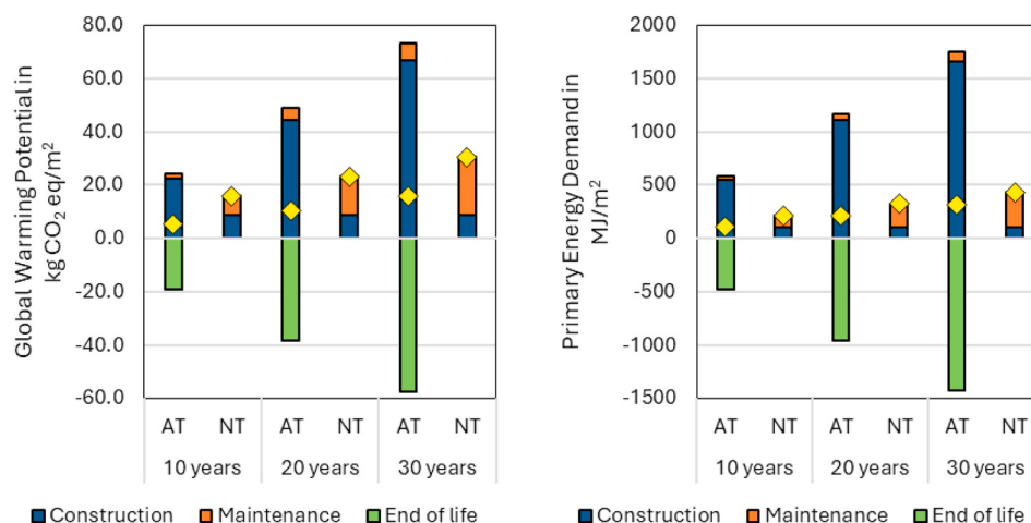
Fig. 3. GWP in kg CO 2 eq/m 2 turf (left) and PED in MJ/m 2 turf (right) for the reference case. The blue bars represent the construction phase, the orange bars represent the maintenance phase, the green bars represent the end-of-life phase, and the yellow diamonds represent the total LCA impact.
