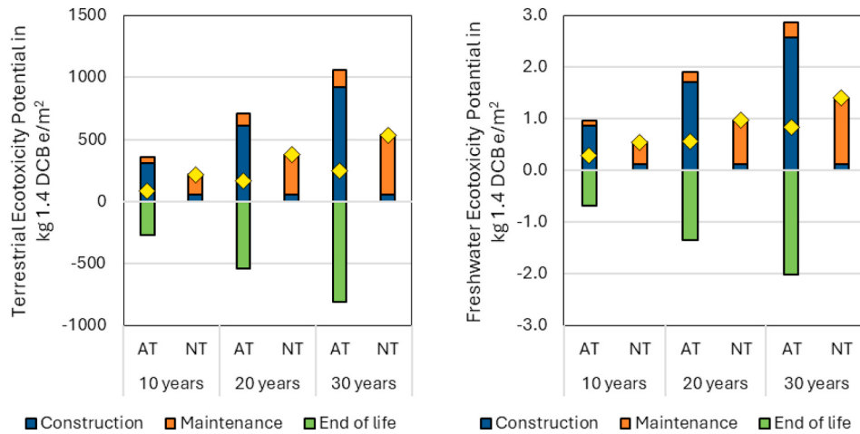
Fig. 5. TEP in kg 1.4 DCB e/m 2 turf (left) and FEP in kg 1.4 DCB e/m 2 turf (right) for the reference case. The blue bars represent the construction phase, the orange bars represent the maintenance phase, the green bars represent the end-of-life phase, and the yellow diamonds represent the total LCA impact.
