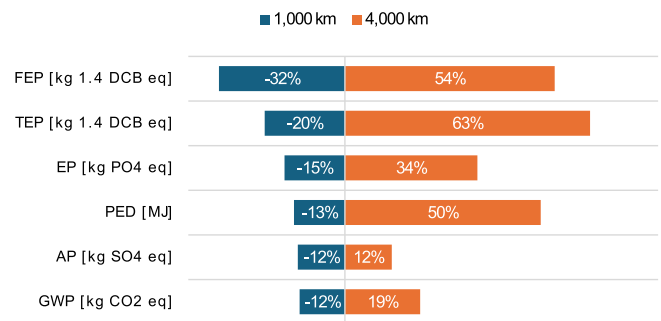
Fig. 6. Environmental impacts are visualized based on various distances from the selected points of AT, considering both shorter and longer distances.
