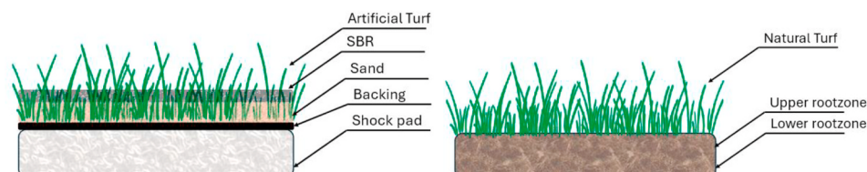
Fig. 1. To the left are the layers of an AT which include a shock pad, backing, sand, SBR and AT. To the right are the layers of a NT which include a lower rootzone, upper rootzone and turf.
