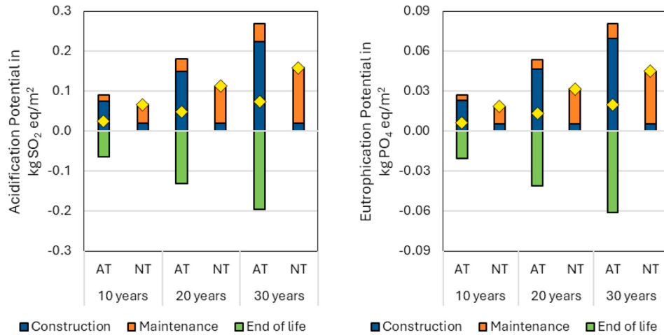
Fig. 4. AP in kg SO 2 eq/m 2 turf (left) and EP in kg PO 4 eq/m 2 turf (right) for the reference case. The blue bars represent the construction phase, the orange bars represent the maintenance phase, the green bars represent the end-of-life phase, and the yellow diamonds represent the total LCA impact.
